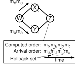
Figure 2: Example: detecting and performing rollback. In this example, we assume all messages originate from node W , and all links have the same expected delay. Thus, the order of the messages are determined by the sequence numbers. We assume messages m_b , m_a , m_d , and m_c have sequence numbers 0, 1, 2, and 3, respectively.
