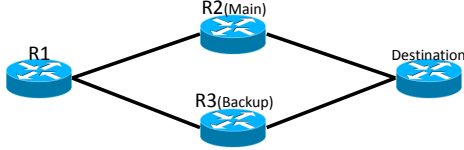
Figure 5: An illustration of the known timing bug in the RIP module of Quagga 0.96.5.
