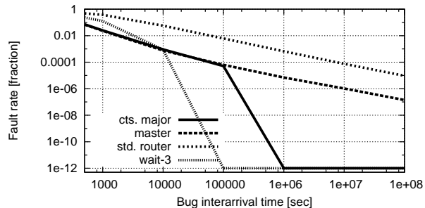
Figure 4: Effect of bug interval on fault rate, holding bug duration fixed at 600 seconds.
